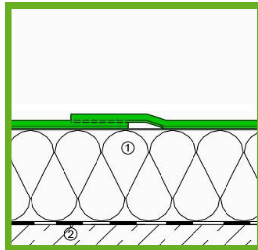
Layer construction: KÖSTER TPO Membrane (green); Insulation (1); Substructure (2)
