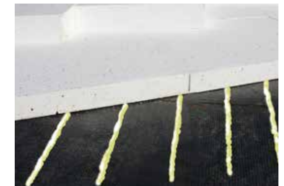
Next, the insulation is adhered. It is recommended to use KÖSTER PUR Membrane Adhesive.
