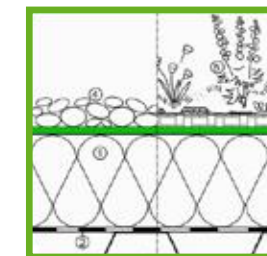
Loose laying with ballast
